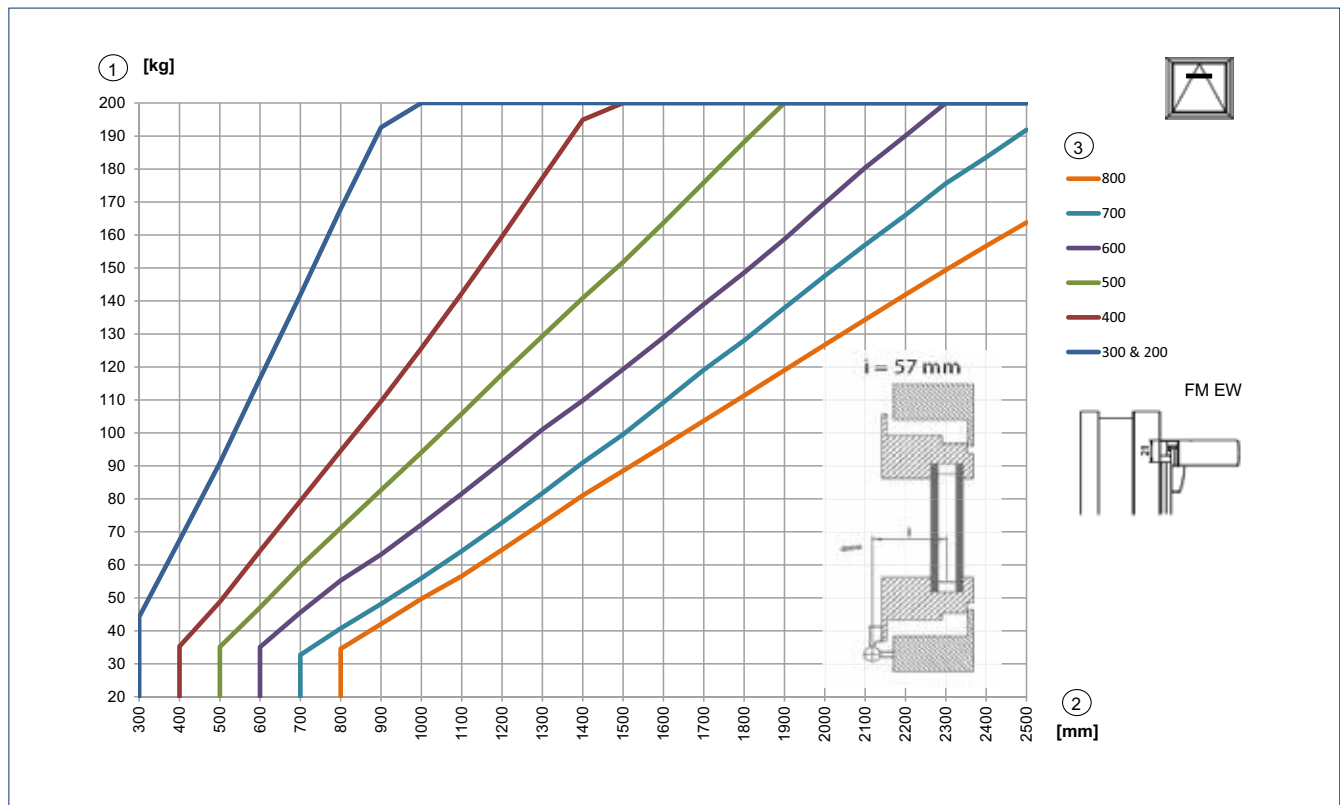
Area of application applies for one Solo drive, for Syncro 2 or Syncro 3 the leaf weight can be doubled or tripled. The details provided by the profile system manufacturer must be heeded. 1 = Leaf weight | 2 = Secondary closing edge | 3 = Stroke [mm]
