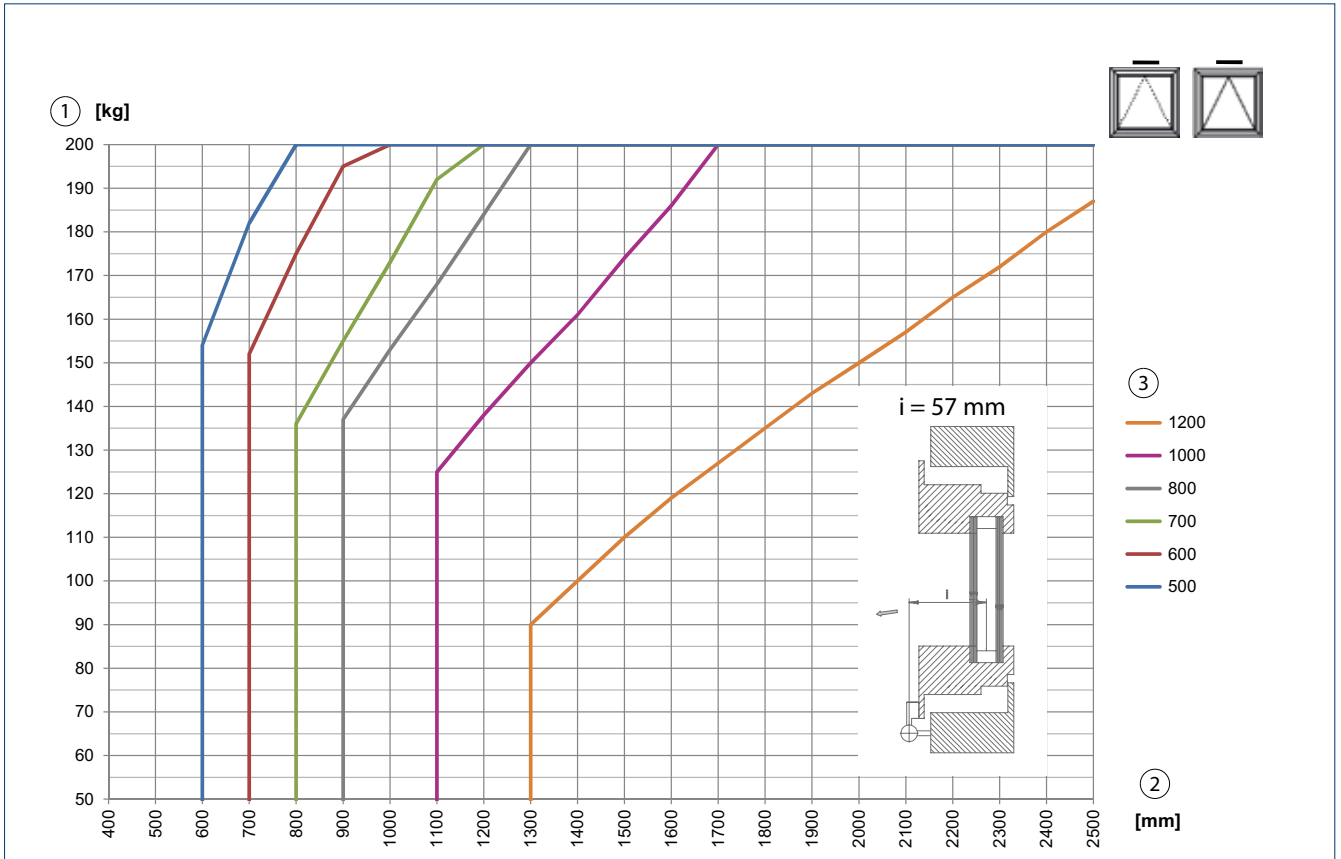
Area of application applies for one Solo drive, for Syncro 2 or Syncro 3 the leaf weight can be doubled or tripled. The details provided by the profile system manufacturer must be heeded. | 1 = Leaf weight | 2 = Secondary closing edge | 3 = Stroke
