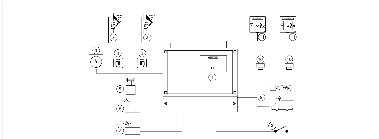
1 = SHEV emergency power supply unit | 2 = Drives for windows and smoke extraction flaps | 3 = Vent switch | 4 = Timer | 5 = Rain/wind control | 6 = Signal window OPEN (optional) | 7 = Signal fault (optional) | 8 = Alarm from external fire alarm system | 9 = Signal alarm (alarm forwarding) (optional) | 10 = Smoke detector and heat detector | 11 = RWA buttons
