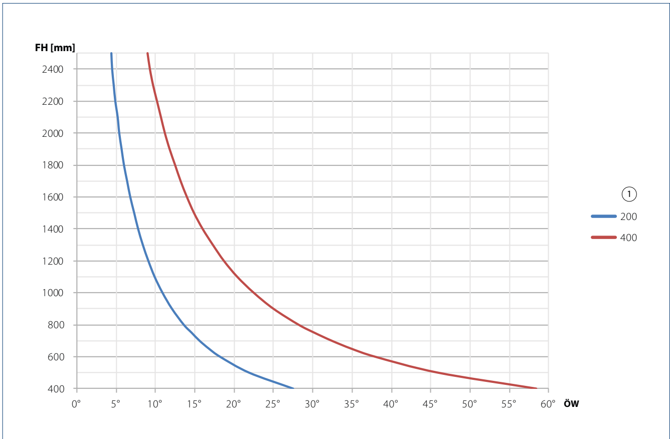
FH = Leaf height | ÖW = Opening angle | 1 = Stroke
