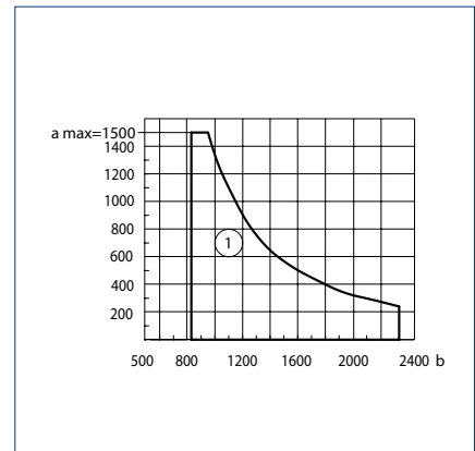
a max. = 1500 mm | b min. = 845 mm | b max. = 2335 mm | 1 = Side-hung window
