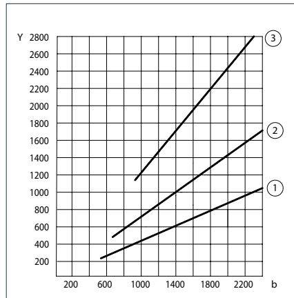
Y = Opening angle (mm) | b = Leaf height (bottom-hung leaf)/Leaf width (side-hung window) (mm) | 1 = Stroke 100 ÖW-25° | 2 = Stroke 150 ÖW-40° | 3 = Stroke 230 ÖW-75°
