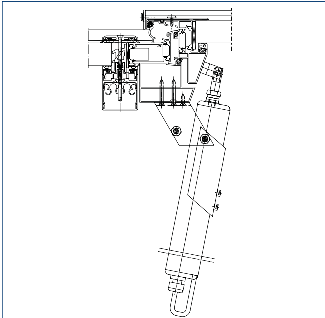
Standard console E 250 NT / E 350 N, incl. standard leaf bracket (ID no. 019032)
