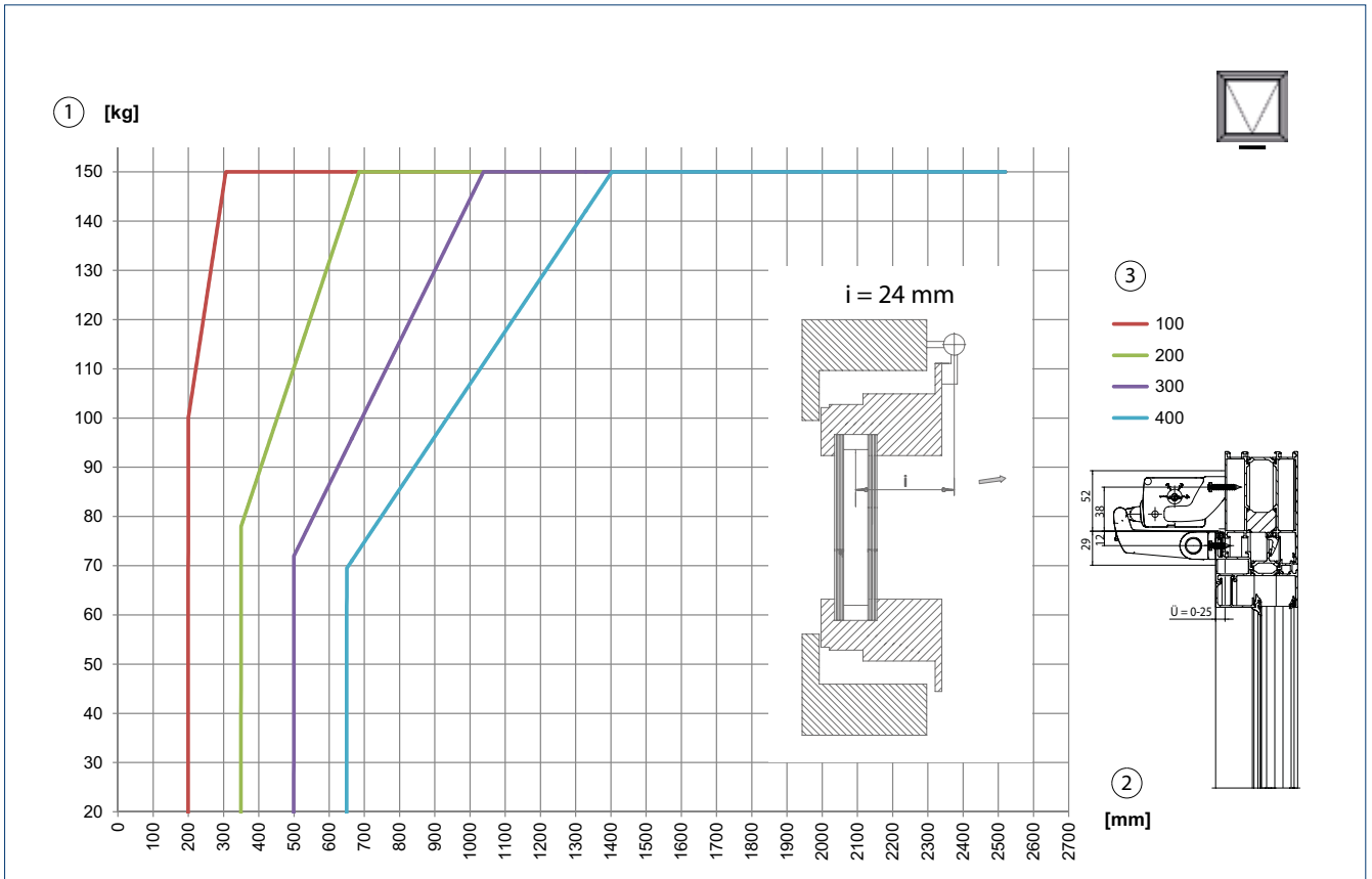
1 = Leaf weight | 2 = Secondary closing edge | 3 = Stroke
