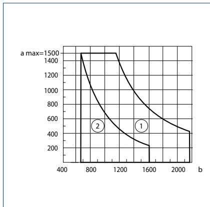
a max. = 1500 mm | b min. = 685 mm | b max. = 2175 mm | 1 = Side-hung window | 2 = Bottom/top-hung window
