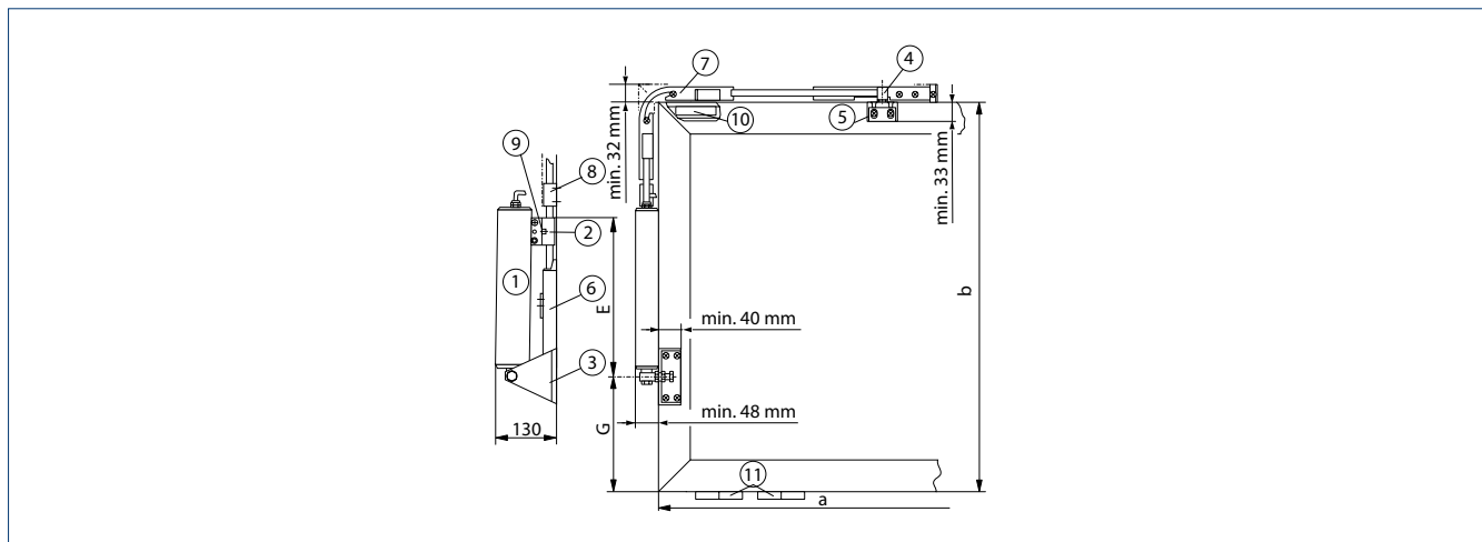
a = Leaf width | b = Leaf height | 1 = E 250 NT electric spindle drive | 2 = Clamping piece | 3 = Toe angle bracket | 4 = Additional locking OL 320 | 5 = Additional bracket complete | 6 = Release spring OL 320 | 7 = Corner transmission OL 320 | 8 = Rod guide OL 320 | 9 = Folding bracket E 250 | 10 = Headstock (on site) - only required for PVC windows | 11 = 2 hinges on the electric drive side (to be provided by customer)
