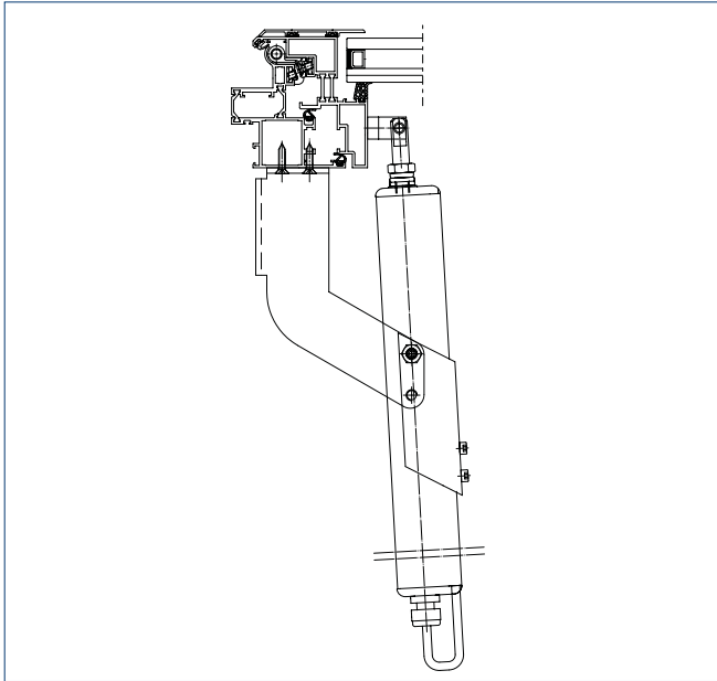
Console INWARD opening E 250 NT / 350 N, incl. standard leaf bracket (ID no. 027218)
