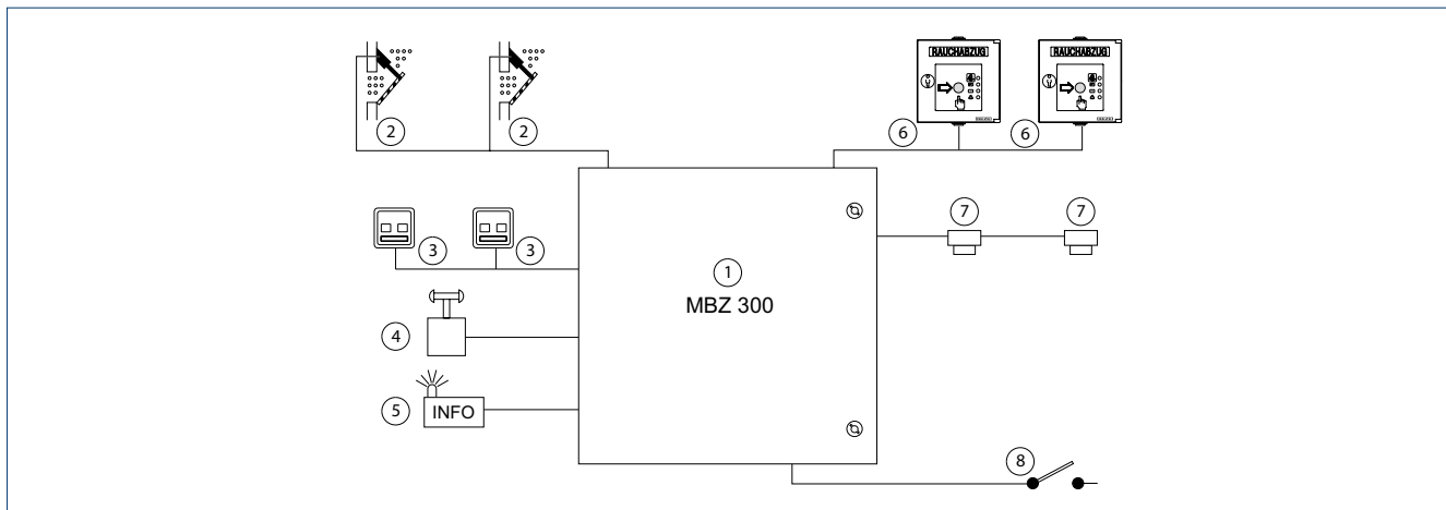
1 = MBZ 300 SHEV modular bus control unit | 2 = Drives of the window and smoke extraction flaps | 3 = Vent switch | 4 = Rain/wind control | 5 = Alarm interference signals | 6 = SHEV button | 7 = Smoke detector and heat detector | 8 = Alarm from external fire alarm system
