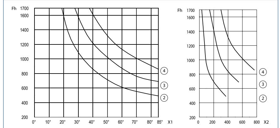
X1 = Opening angle | X2 = Space needed for swivel (mm) | Fh = Leaf height (mm) | 2 = Stroke 500 | 3 = Stroke 750 | 4 = Stroke 1000
