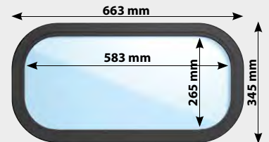
Rounded corners (r=100 mm), excellent insulation value
