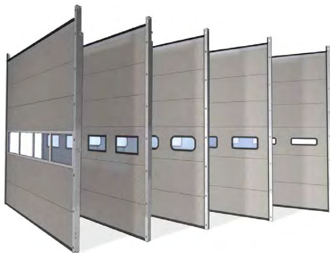
U-value Thermo 40 mm overhead door: 5,000 x 5,000 mm: 1.02 \text{ W/m}^2\text{K}
