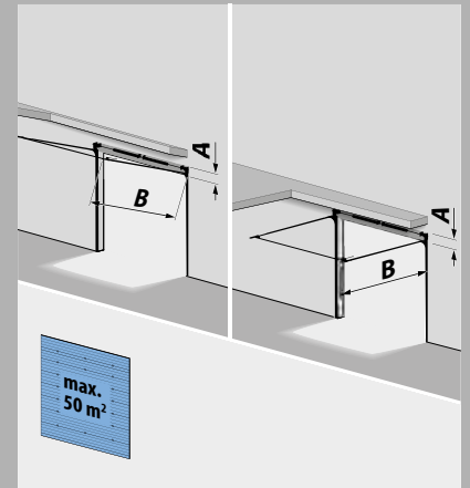
T 450 (B45), standard rail system (comes standard)
